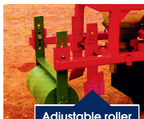
Adjustable roller height to re-compact soil
